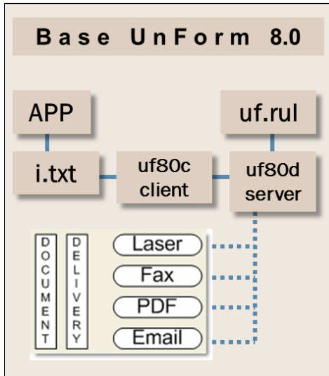
A simple depiction of the Base UnForm flow of processing
